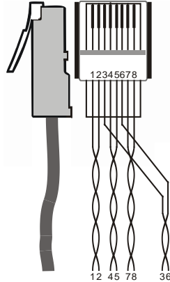
Figure 15: CAT 5 PINOUT
