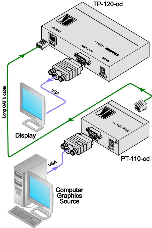
Figure 3: Connecting the PT-110-od to the TP-120-od
