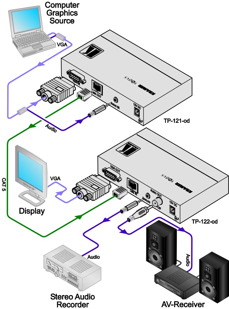
Figure 6: Connecting the TP-121-od and the TP-122-od
